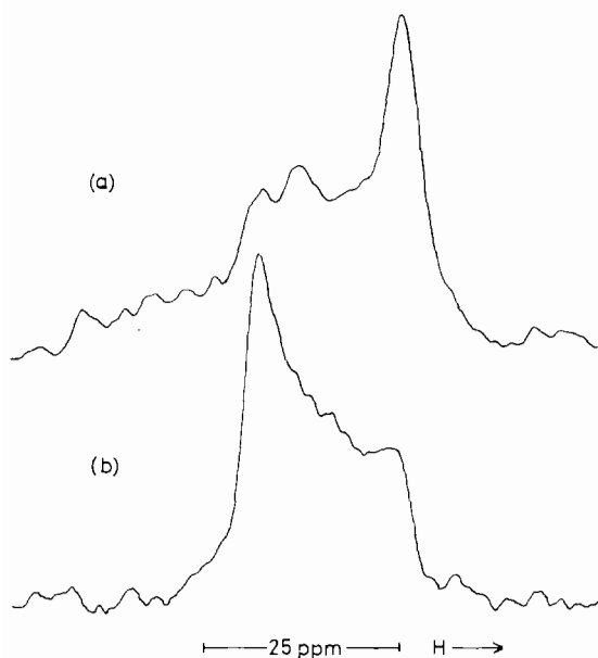
Fig. 5. 36.4 MHz ^{31}\text{P} NMR spectra of aqueous dispersions of 18 : 1 c /18 : 1 c phosphatidylethanolamine (a) in the absence and (b) in the presence of equimolar cholesterol ( T = 3^\circ\text{C} ). All dispersions contained 25 mM Tris/acetic acid (pH 7.0) and 2 mM EDTA.
