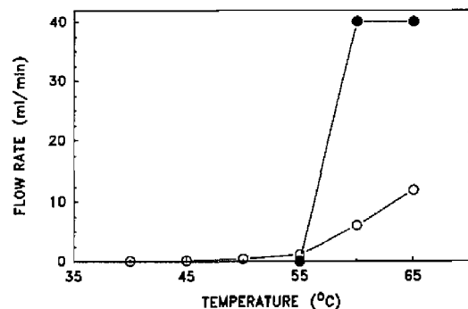
Fig. 1. Effect of temperature on extrusion of DSPC (●) and DSPC/chol (55:45 mol ratio) (○) MLVs. MLVs were initially hydrated at 15 \text{ mg} \cdot \text{ml}^{-1} in 150 mM NaCl, 20 mM HEPES buffer (pH 7.4) at 65^\circ\text{C} and equilibrated for 15 min. Aliquots (2 ml) were equilibrated for 15 min at the appropriate temperature in the extrusion device and subsequently extruded at 3500 kPa.
