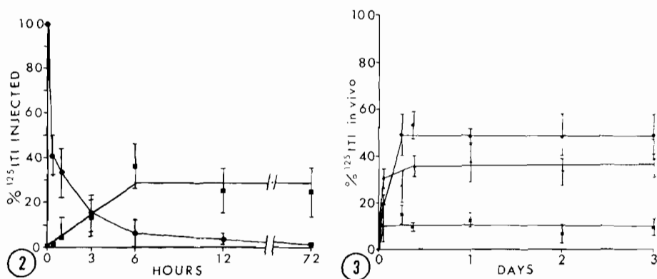
Figure 2. Clearance of ^{125}\text{I} ITI entrapped in EPC-cholesterol (1:1) LUV systems from the (rat) circulation (●) and subsequent excretion in the urine (■). The LUV's were prepared as indicated in Methods and were injected into the tail vein of 150-175 g female Wistar rats at a dose level of 0.5 \mu\text{mol} phospholipid in 100 \mu\text{l} HBS. Urine was collected in metabolic cages. Blood was withdrawn and the animals sacrificed at indicated times and the total amount of ^{125}\text{I} ITI in the blood calculated assuming 4.9 \text{ ml} blood per 100 \text{ g} rat. Results are expressed as percentages of the total ^{125}\text{I} ITI injected \pm s.e. ( n = 4 ).
