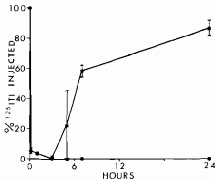
Figure 1. Clearance of free ^{125}\text{I} -tyraminyl-inulin ( ^{125}\text{I} ITI) from the (rat) circulation (●) and subsequent excretion in the urine (■). Female Wistar rats were injected via the tail vein with 1 \mu\text{Ci} ^{125}\text{I} ITI in 200 \mu\text{l} HBS. Urine was collected in metabolic cages. The animals were sacrificed at the times indicated. Recoveries of blood averaged 80% assuming 4.9 ml blood per 100 g rat. Results are expressed as percentages of the total ^{125}\text{I} ITI injected \pm s.e. (n = 3).
