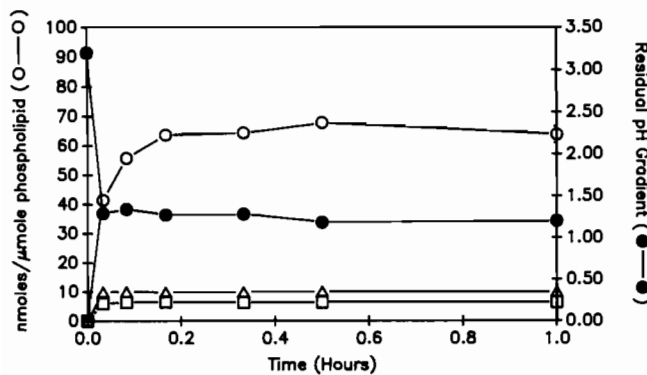
FIGURE 1 Time course (O) of uptake of lysine methyl ester into 100 nm EPC vesicles (3.8 mM) exhibiting a \Delta\text{pH} ( \text{pH}_i = 4.0 ; \text{pH}_o = 7.5 ). Control vesicles with no \Delta\text{pH} ( \Delta , \text{pH}_i = \text{pH}_o = 7.5 ; \square , \text{pH}_i = \text{pH}_o = 4.0 ) were also tested. Uptake was conducted at 20^\circ\text{C} , and the initial external concentration of lysine methyl ester was 1.3 mM.
