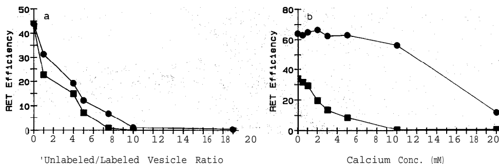
Fig. 8. Effect of calcium and pH on fusion of DOPE/N-succinyl-DOPE vesicles. (a) resonance energy transfer efficiency was monitored by incubating DOPE/N-succinyl-DOPE (7: 3, mol ratio) vesicles containing 1 mol% of N-NBD-PE and 0.5 mol% N-Rho-PE in the presence of increasing amounts of unlabeled DOPE/N-succinyl-DOPE vesicles in pH 7.4 (●) and 4.0 (■) buffers containing 20 mM Ca. (b) Calcium titration of fusion was done at an unlabeled/labeled vesicle ratio of 10 at pH 7.4 (○) and pH 4.0 (●). The reaction was stopped after a 30 min incubation by the addition of 2-fold molar excess EDTA (adjusted to pH 7.4) and resonance energy transfer efficiency was determined.
