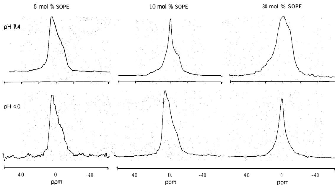
Fig. 7. Effect of pH on bilayer stabilization of DOPE by N-succinyl-DOPE. 81.0 MHz ^{31}\text{P} -NMR spectra were obtained from aqueous dispersions of DOPE containing 5, 10, and 30 mol% N-succinyl-DOPE at pH 7.4 and 4.0. The pH was adjusted by addition of aliquots from 100 mM HCl stock solutions to the lipid dispersions followed by three freeze-thaw cycles.
