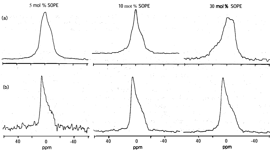
Fig. 5. Influence of calcium on DOPE/N-succinyl-DOPE mixtures. 81.0 MHz ^{31}\text{P} -NMR spectra obtained at 30 ° C from aqueous dispersions of DOPE containing 5, 10, and 30 mol% N-succinyl-DOPE in the absence (a) and presence (b) of \text{Ca}^{2+} . Calcium (equimolar with respect to N-succinyl-DOPE) was added and the samples were freeze-thawed three times to equilibrate the ions across the membranes.
