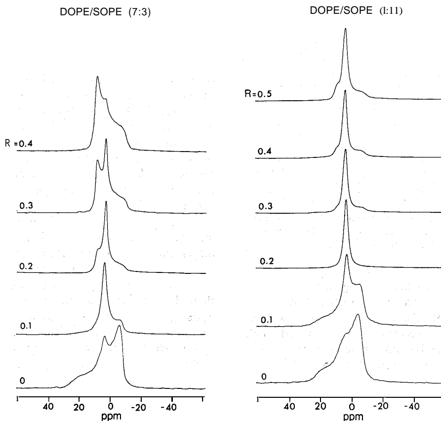
Fig. 6. Calcium titration on DOPE/ N -succinyl-DOPE mixtures containing 30 and 50 mol% N -succinyl-DOPE. 81.0 MHz ^{31}\text{P} -NMR spectra at 30 ° C were obtained from aqueous dispersions of liposomes. The ratio, R , refers to the molar ratio of calcium to N -succinyl-DOPE where the divalent cation was added to the hydrated lipid systems as aliquots from a 100 mM stock solution. The calcium ionophore, A23187, was added at 0.1 mol% to aid calcium ion equilibration and the samples were freeze-thawed two times.
