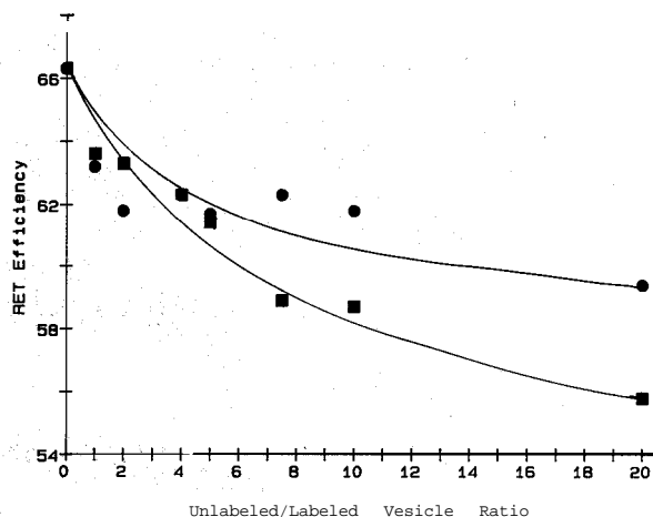
Fig. 3. Effect of pH on fusion of pure N-succinyl-DOPE vesicles in the presence of \text{Ca}^{2+} . Fluorescence resonance-energy transfer was monitored by incubating N-succinyl-DOPE vesicles containing 1 mol% N-NBD-PE and 0.5 mol% N-Rho-PE with increasing concentrations of unlabeled vesicles at pH 7.4 and pH 4.0 in the presence of 20 mM \text{Ca}^{2+} . The resonance energy transfer efficiency of energy transfer fusion at pH 7.4 (●) and at pH 4.0 (■) was measured as described in Methods.
